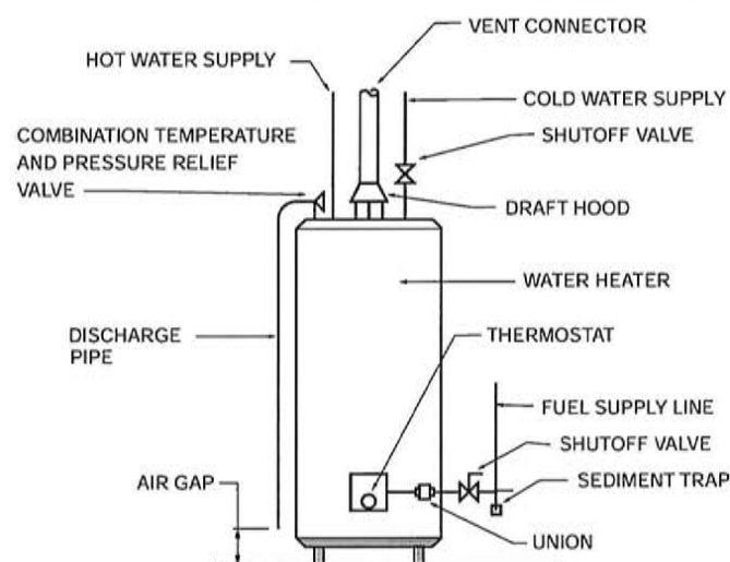
Commentary Figure 505.4 WATER HEATER INSTALLATION REQUIREMENTS
