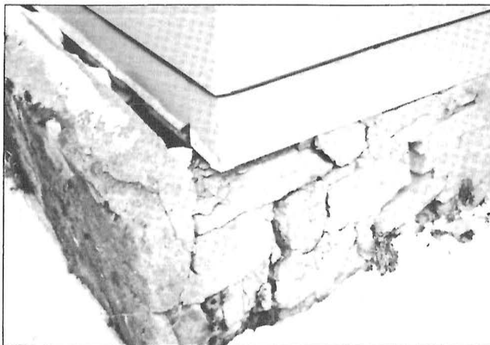
Commentary Figure 304.5 MAJOR DAMAGE TO A FOUNDATION WALL
