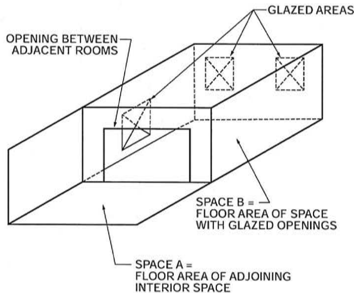
Commentary Figure 402.1(3) NATURAL LIGHT FROM ADJACENT SPACE
