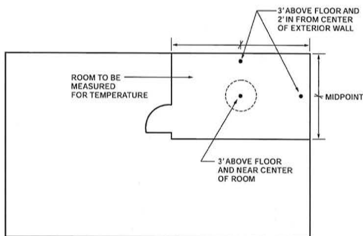
Commentary Figure 602.5 ROOM TEMPERATURE MEASUREMENTS
